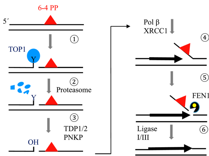
Figure 24.6. A DNA repair problem arising when TOP1 encounters a DNA lesion, in this case a 6-4 pyrimidine dimer (Saha et al., 2020). In step 1 , TOP1 has cleaved the DNA strand adjacent to a 6-4 PP and has bound to one end of the break by way of a tyrosine (Y) (see Chapter 11). The TOP1 is now trapped and cannot proceed. In step 2 , a proteasome cuts away most of the trapped TOP1 protein. Step 3 removes the remaining peptide, including the Y, leaving a 3'OH. In steps 4-6 , long-patch BER comes into play and completes the repair, as in Figure 24.5.
