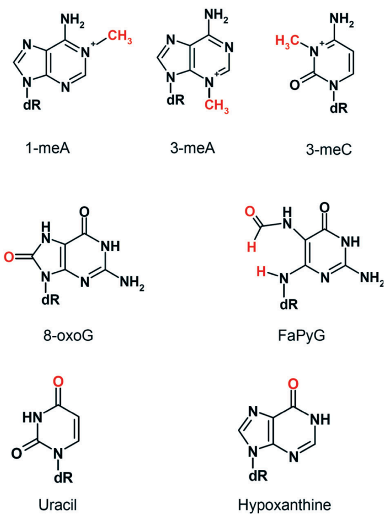
Figure 24.3. Some of the chemically altered bases that BER is capable of removing from damaged DNA (Robertson et al., 2009).
