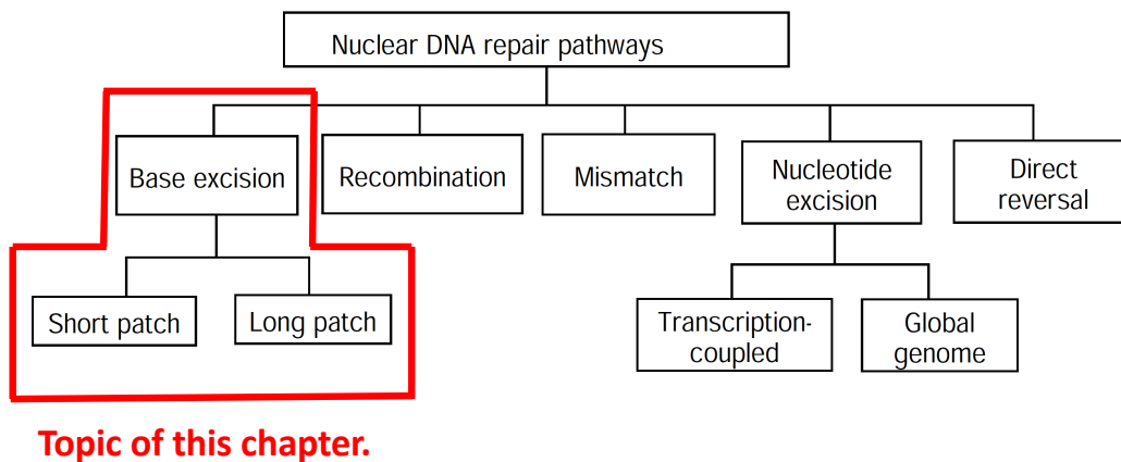
Figure 24.1. The topic of this chapter, base excision repair (BER), in relation to the other DNA repair pathways in the cell nucleus. From (Kohn and Bohr, 2001).
