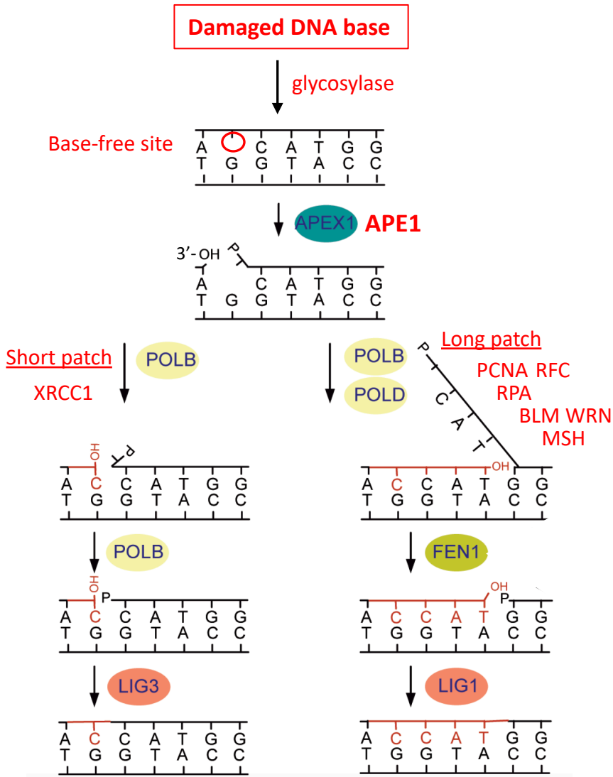
Figure 24.5. Steps in the repair of base-free sites after removal of an altered or damaged base from DNA where there is a damaged base. ((Robertson et al. , 2009) with labels in red added.)
